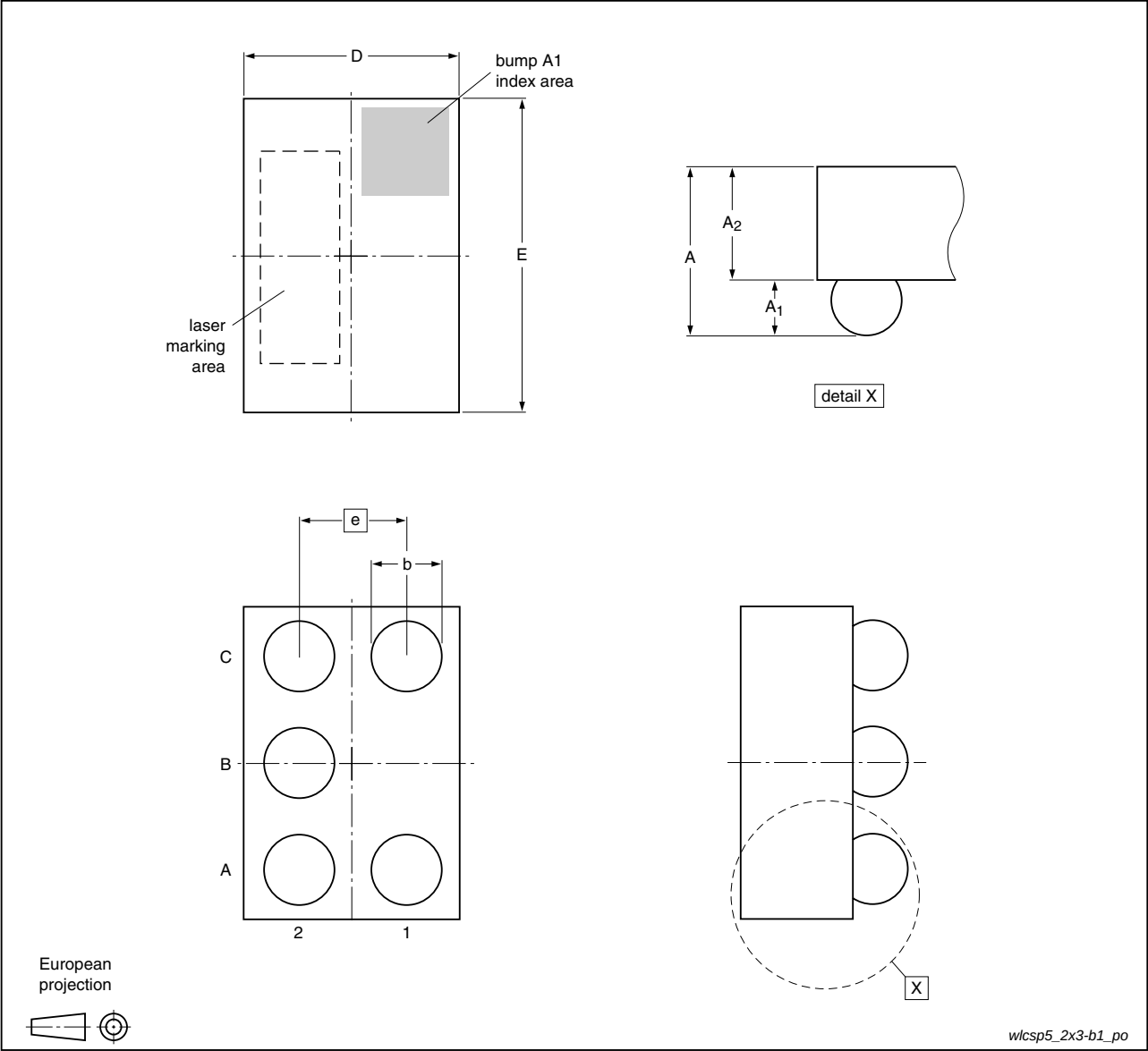
Fig 9. Package outline IP5311CX5/LF (WLCSP5)
